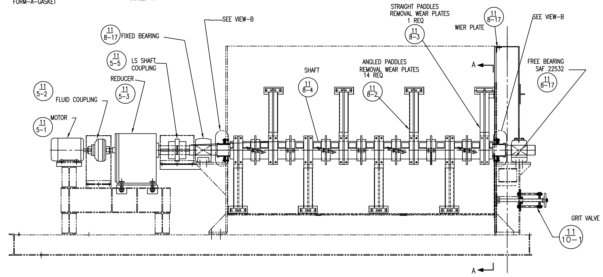
MAIN CHAMBER PARTS LOCATOR
