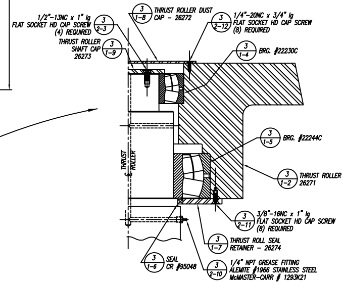
ENLARGED BEARING ASSEMBLY
